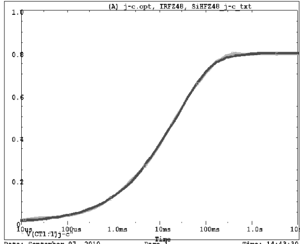
IRFZ48, SiHFZ48 Tank j-c Temperature: 27.0
