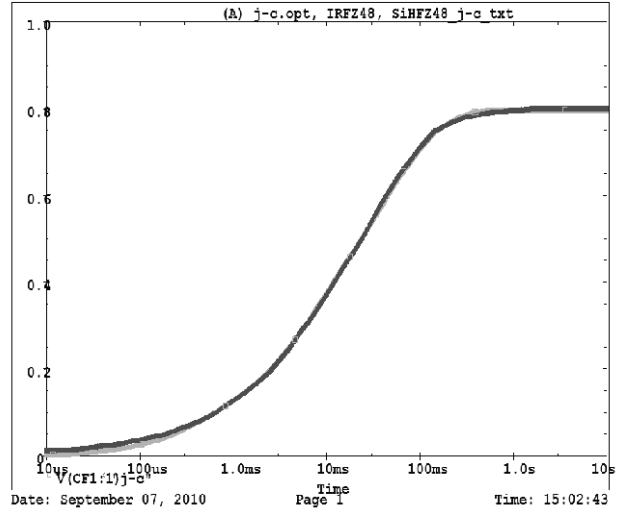
IRFZ48, SiHFZ48 Filter j-c Temperature: 27.0
